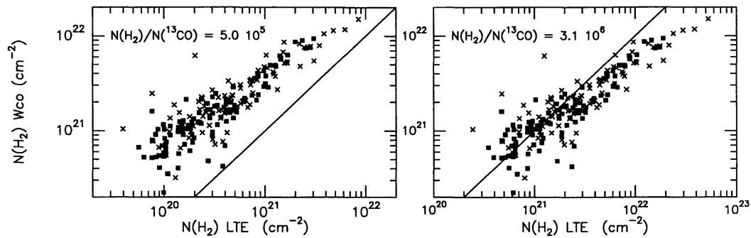
Figure 2. Comparison of column densities of H_2 calculated via N_{Wco} = X W_{CO} , with N_{lte} . The filled squares are IRAM 30-m data of the WB283 cloud and the crosses SEST data of several other FOG clouds. Left-hand panel: used local abundance ratio N(H_2)/N(^{13}CO) ; right-hand panel: used abundance ratio at R=17 kpc, extrapolated from the gradients given by [16]. In both panels X=2.3 \cdot 10^{20} \text{ cm}^{-2}(\text{Kkms}^{-1})^{-1} , i.e. the value appropriate for the inner Galaxy, and the drawn line is for equal column densities. When taking the abundance gradients into account N_{Wco} \approx N_{lte} for X in the far-outer Galaxy equal to the inner Galaxy value.
