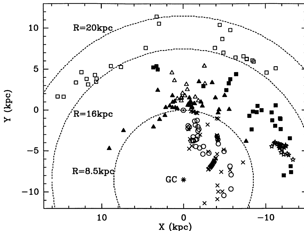
Figure 1. Distribution of the molecular clouds used in the analysis. The Sun is at (X,Y)=(0,0) and indicated by \odot ; the galactic center is at (X,Y)=(0,-8.5) . Dashed circle segments indicate R = 8.5, 16 , and 20 kpc respectively. The individual data sets are distinguished by different symbols: [5] (open squares), [8] (filled squares), [9] (open triangles), [10] (filled triangles), [11] (asterisks), [12] (circles), [13] (crosses).
