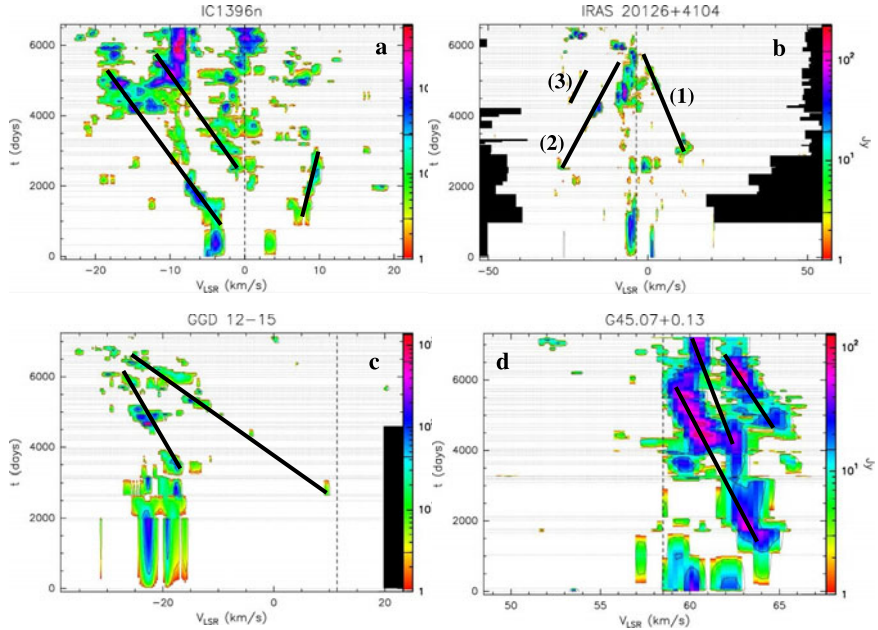
Figure 3. Velocity gradients in VtF-diagrams. Drawn lines indicate possible velocity drifts of maser components. a. IC1396N b. IRAS20126+4104 c. GGD12-15 d. G45.07+0.13. (See the online version for colour contours).
