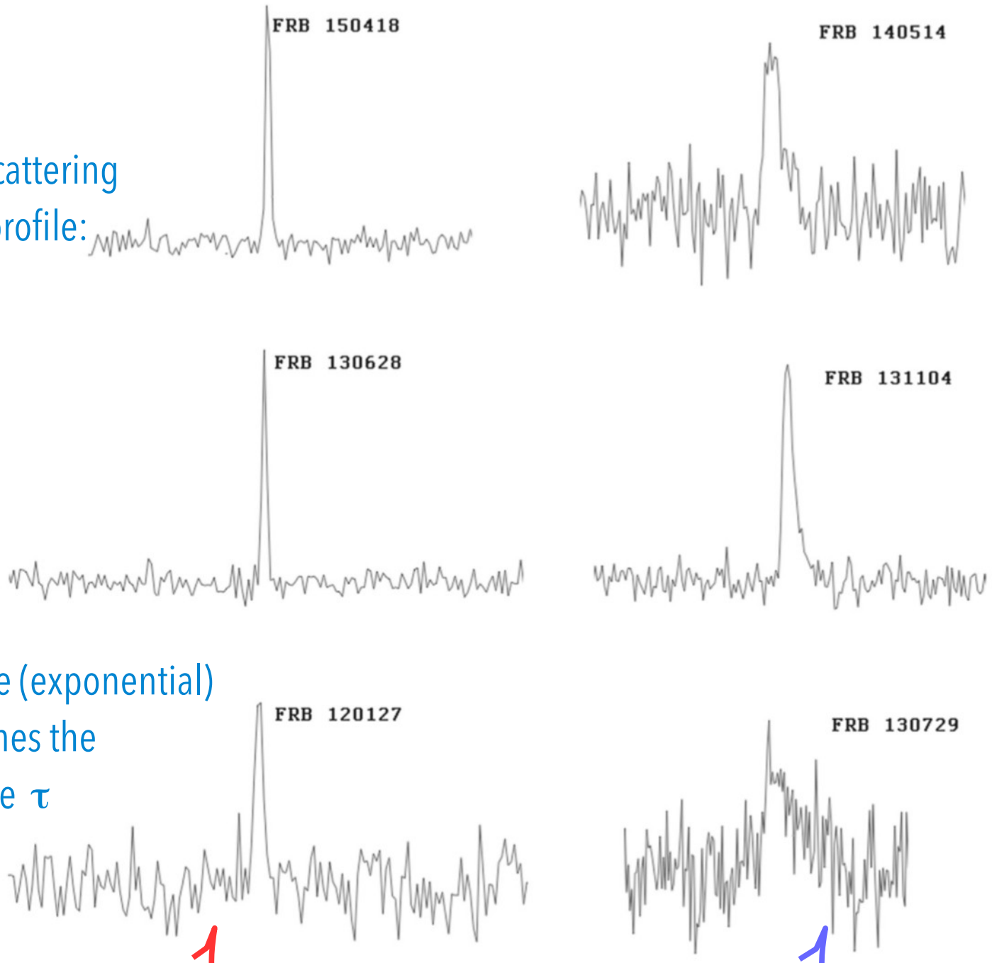
Figure 3. FRBs with no scattering are shown in the left panel and FRBs with scattering are shown in the right panel. The horizontal time scale is 60 ms for each profile.
