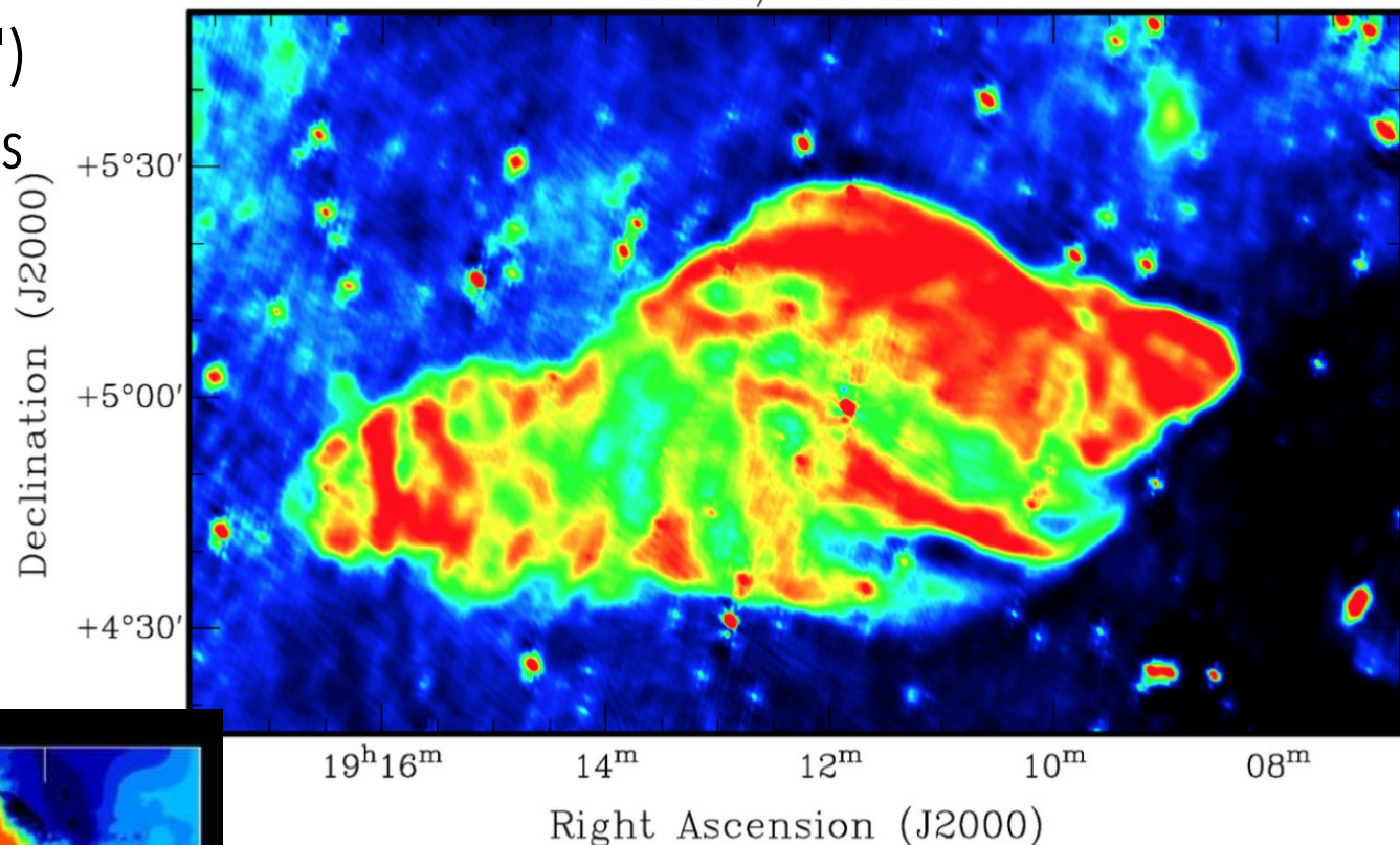
SS433/W50 HBA
