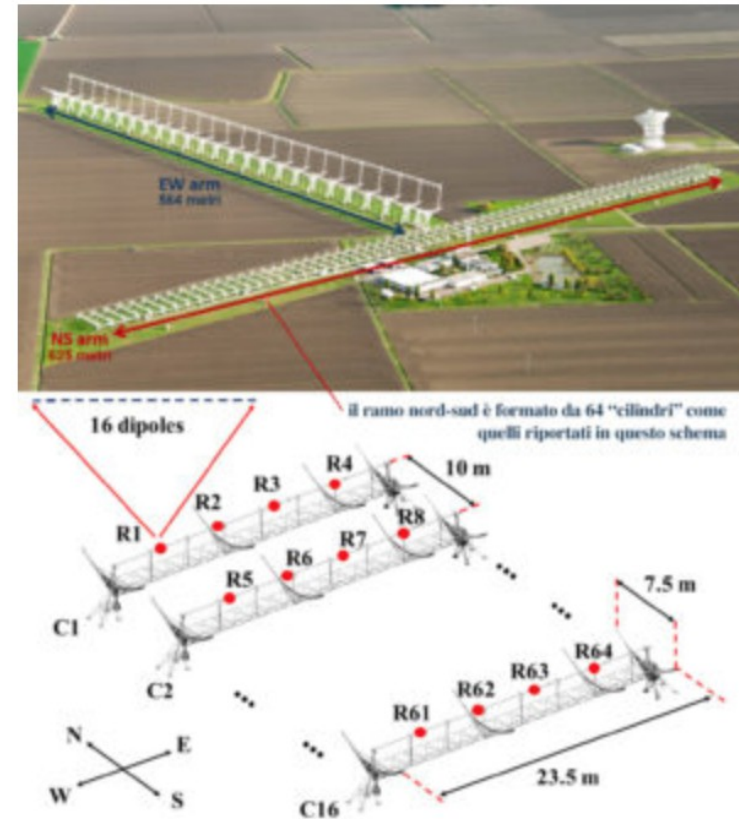
Above, aerial view of the Medicina Station, with the two perpendicular branches of the Northern Cross. Below, diagram of the "cylinders" that form the north-south branch. Source: N. Locatelli et al. Mnras, 2020
