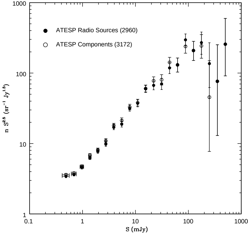
Fig. 4. Normalized 1.4 GHz differential source counts derived from the ATESP catalogue. Filled circles refer to the ATESP radio source catalogue (2960 distinct objects). Empty circles refer to the list of all the ATESP components (3172 entries). Horizontal bars represent 1\sigma errors in the measured total flux. Vertical bars represent Poissonian errors
