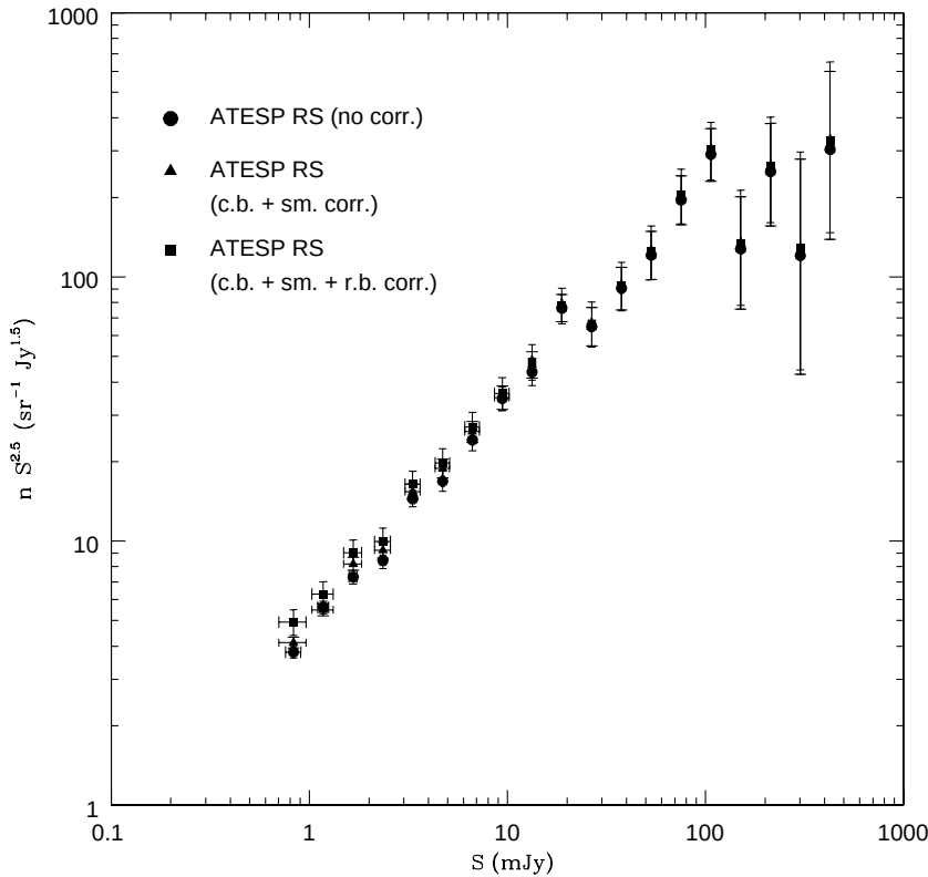
Fig. 5. Normalized 1.4 GHz differential source counts derived from the ATESP catalogue (multiple sources are counted as one object). The source counts are plotted before (filled circles, same as shown in Fig. 4) and after correcting for clean bias and bandwidth smearing (filled triangles). In the latter case horizontal bars represent 1\sigma errors in the corrected total flux. Filled squares represent the counts obtained once the resolution bias is also taken into account. Vertical bars include here the uncertainty in the resolution bias correction. In all cases the counts have been derived down to 0.70 mJy (instead of 0.41 mJy), in order to avoid the incompleteness effects introduced by the flux corrections
