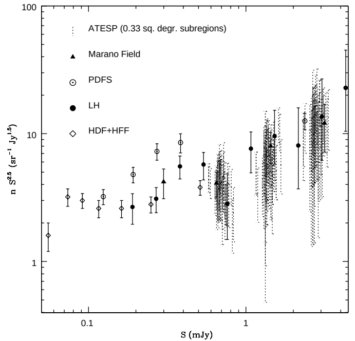
Fig. 8. Normalized 1.4 GHz differential source counts for 0.33 sq. degr. ATESP sub-regions (dotted 1\sigma Poissonian error bars). For consistency these counts are compared only to the ones obtained from the surveys covering areas of the same order of magnitude (a fraction of sq. degr.): the PDFS (circled dots), the Marano Field (triangles), the HDF+HFF (diamonds) and the Lockman Hole (filled circles). The ATESP counts are not corrected for clean bias, bandwidth smearing and resolution bias (Horizontal error bars have not been drawn to prevent overcrowding)
