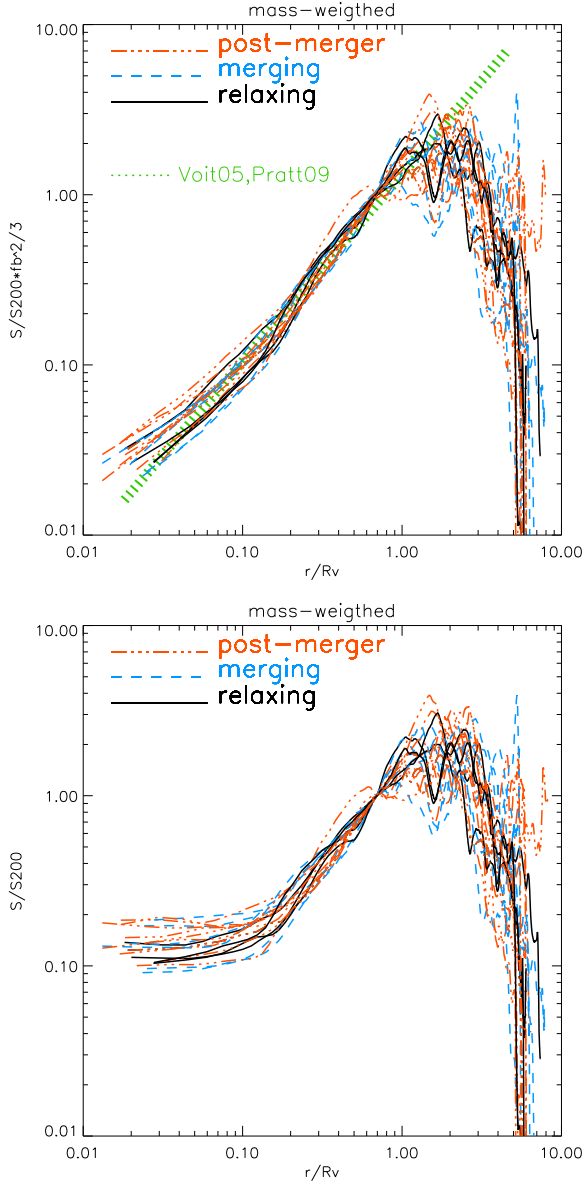
Figure 10: Top panel: gas entropy radial profiles normalized by the baryon fraction within the same radius, as suggested by Pratt et al.(2009). The additional line is the best fit from Voit et al.(2005). Bottom panel: gas entropy profiles normalized by their value at r_{500} .
