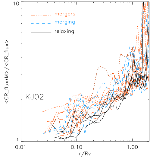
Figure 15: Profiles of volume-weighted mean Mach number (top panel), thermal flux weighted mean Mach number (middle panel), CR-flux weighted mean Mach using a Kang & Jones (2002) injection model (lower panel).
