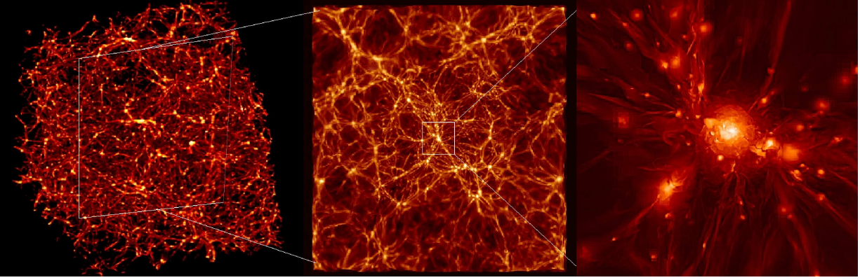
Figure 2: Left : 3-D rendering of gas matter within a 187 Mpc/h computational box at z = 0 . Center : slice of thickness \approx 20 Mpc/h and with the size of 187 Mpc/h centered in the AMR region. The renderings are done with Visivo (Comparato et al. 2007, http://visivo.cineca.it ). Right : 3-D distribution of Dark Matter density inside the AMR region (the side of the image is \approx 8 Mpc/h ) at z = 0 .
