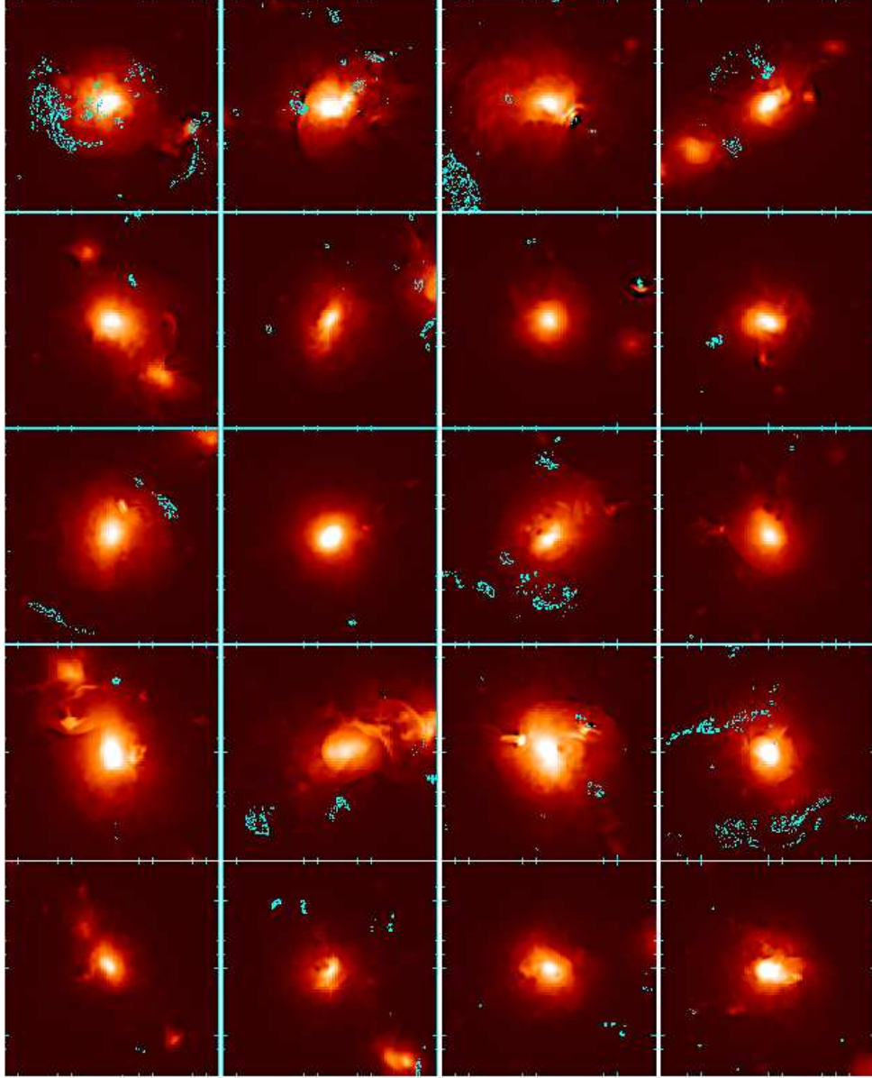
Figure 20: Colors: projected X-ray bolometric luminosity for all clusters in the sample (the color table is as in Fig.16). Contours: energy flux for CR accelerated at shocks, for E \approx 1\text{GeV} particles. The contours range for about 2 order of magnitude in flux, and they are spaced by \Delta\log(E) = 0.2 .
