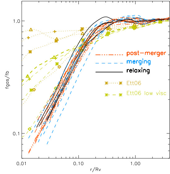
Figure 9: Radial profiles of gas baryon fraction for the clusters in the sample at z = 0 . The additional lines are for 4 galaxy clusters produced with GADGET2, with standard viscosity (dotted lines) or a reduced viscosity scheme (dashed lines), as reported in Ettori et al.(2006).
